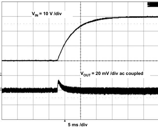
Figure 29. Line Transient
